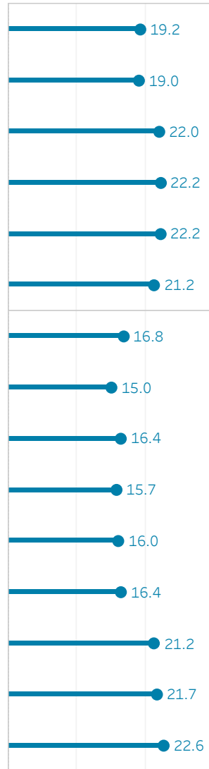
Averages
